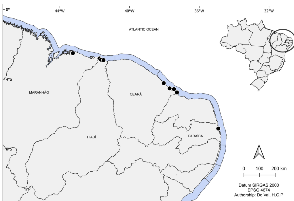
Figure 1. Map of the northeast Brazilian coast, indicating the Greater Caribbean manatee ( Trichechus manatus manatus ) stranding sites in black dots and the species distribution in light blue (IUCN, 2023).
